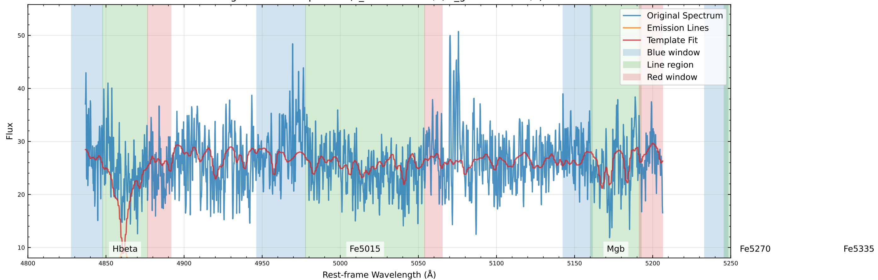
Original Data Comparison (v_star=24.1 km/s, v_gas=-11.7 km/s)
