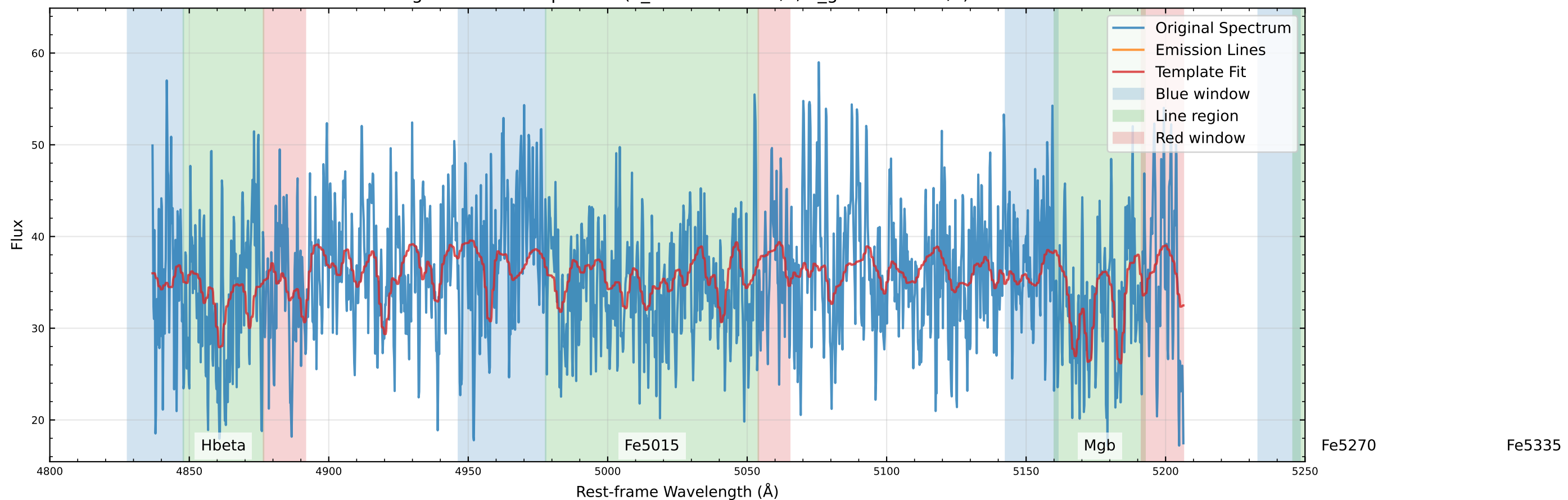
Original Data Comparison (v_star=-10.1 km/s, v_gas=25.4 km/s)
