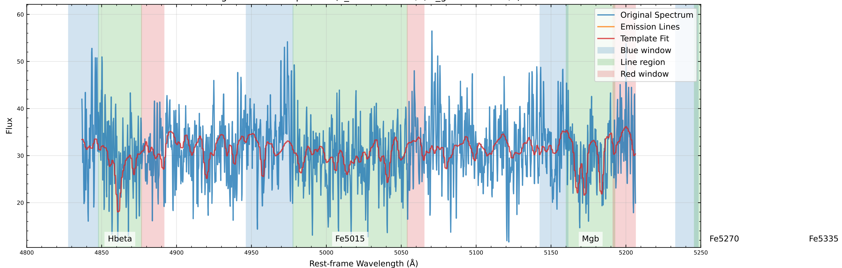
Original Data Comparison (v_star=19.1 km/s, v_gas=-55.1 km/s)
