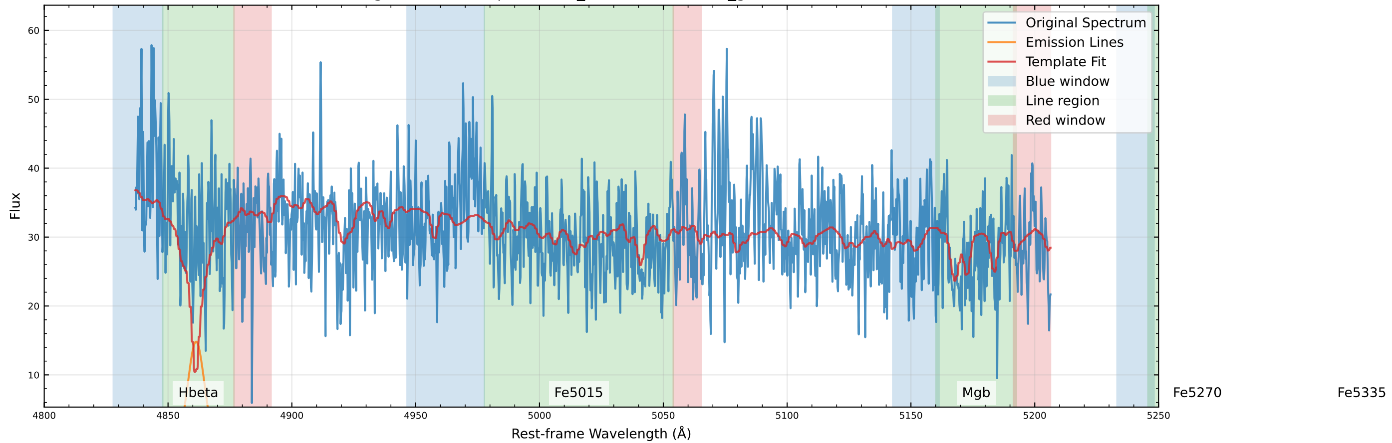
Original Data Comparison (v_star=14.0 km/s, v_gas=7.4 km/s)
