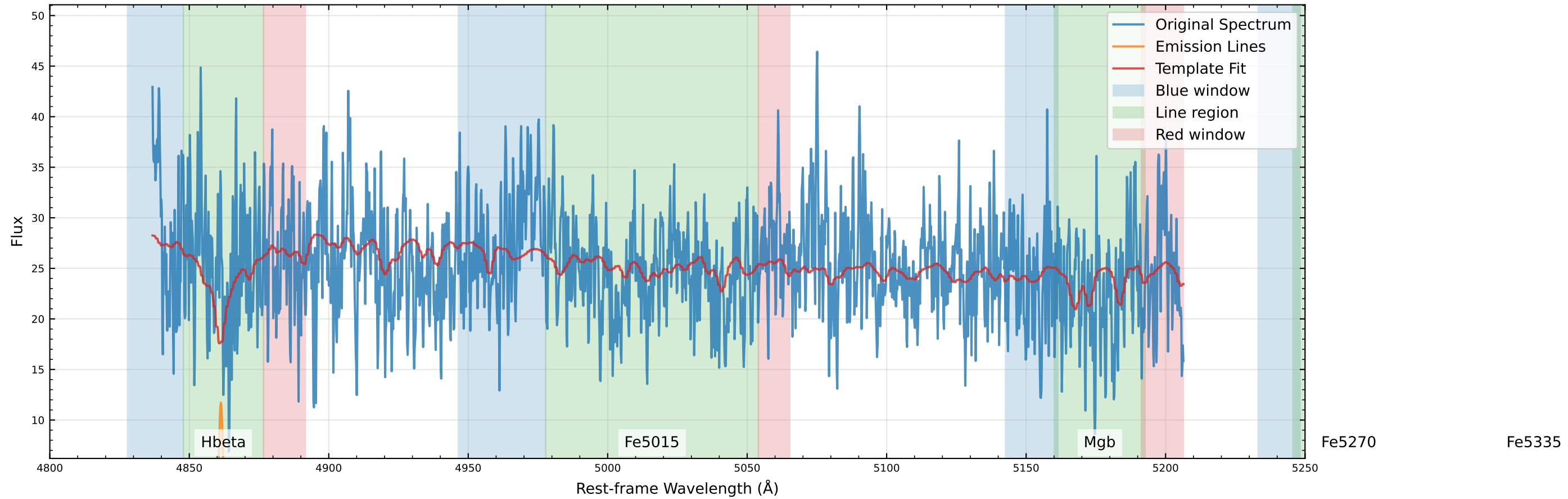
Original Data Comparison (v_star=15.5 km/s, v_gas=-27.2 km/s)
