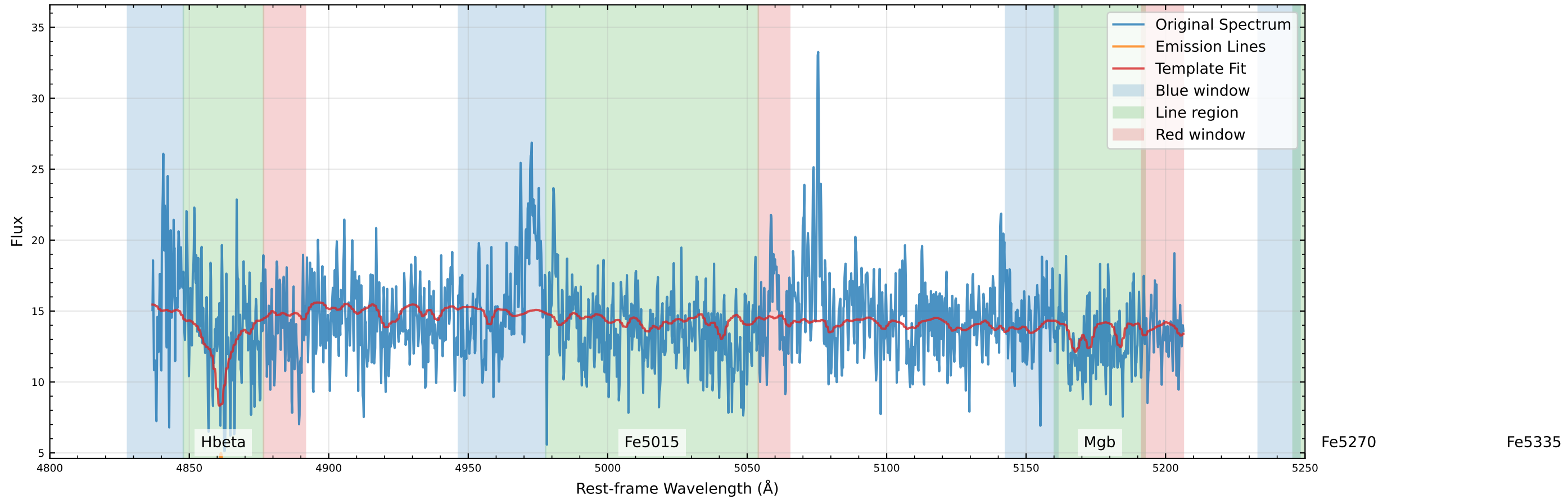
Original Data Comparison (v_star=48.4 km/s, v_gas=-13.2 km/s)
