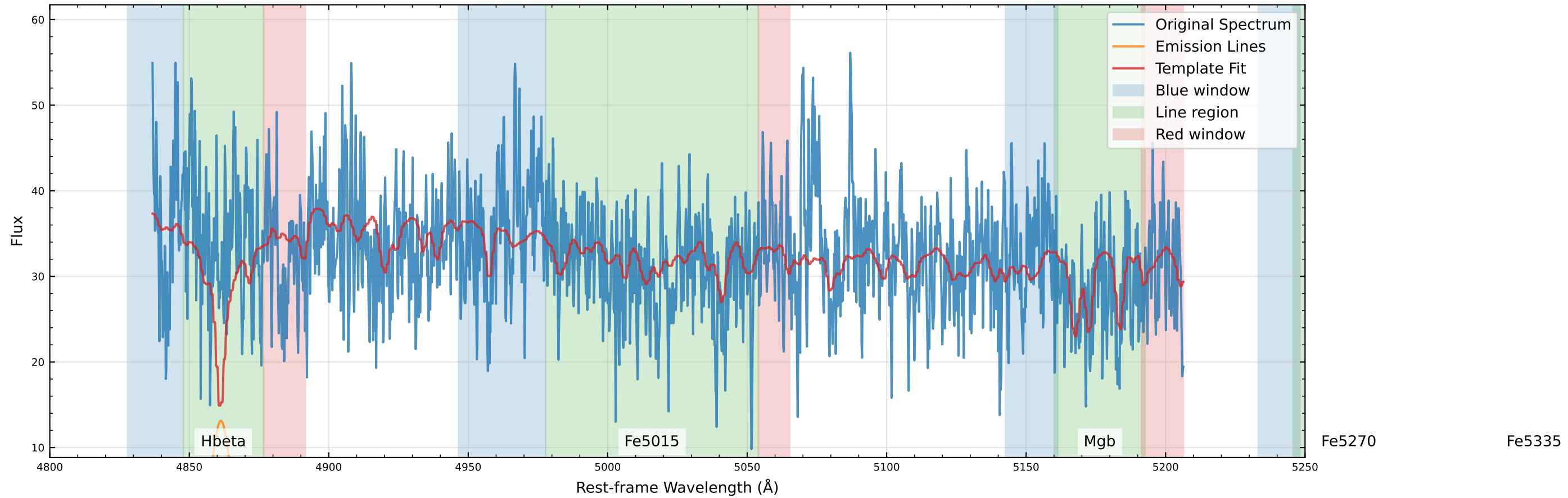
Original Data Comparison (v_star=-33.3 km/s, v_gas=41.6 km/s)
