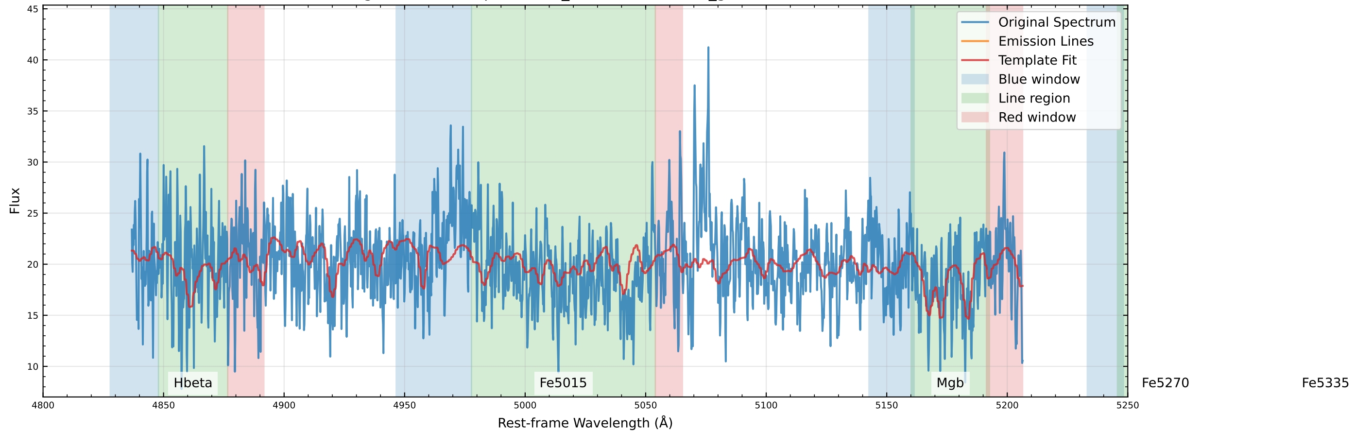
Original Data Comparison (v_star=26.4 km/s, v_gas=4.4 km/s)
