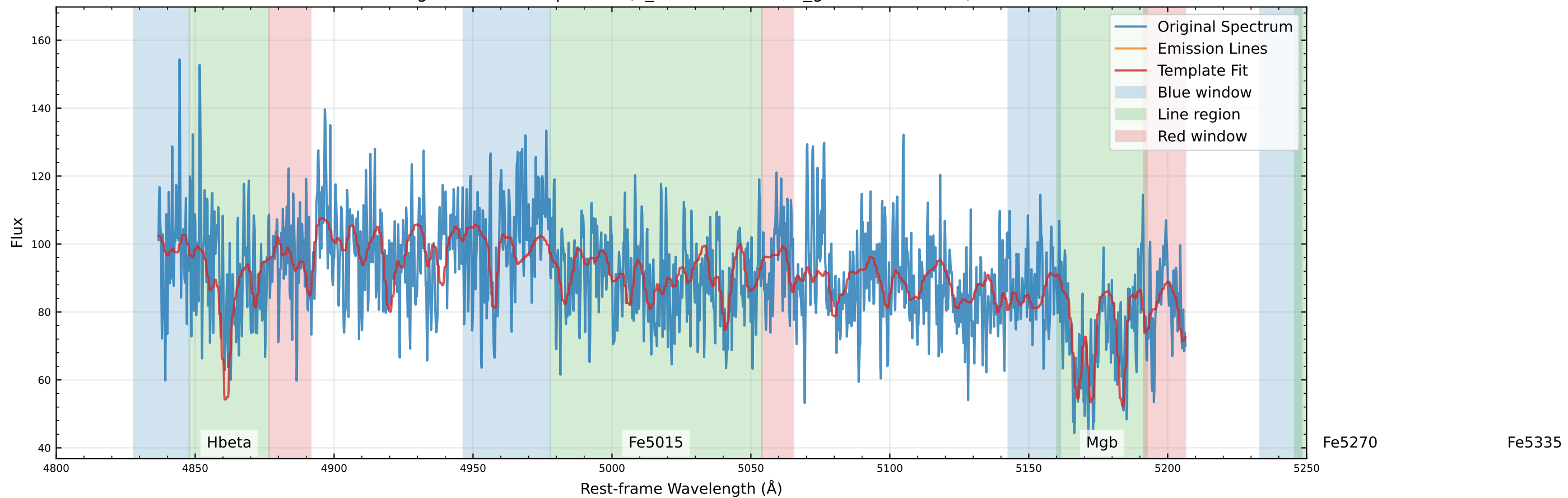
Original Data Comparison (v_star=8.0 km/s, v_gas=-127.3 km/s)
