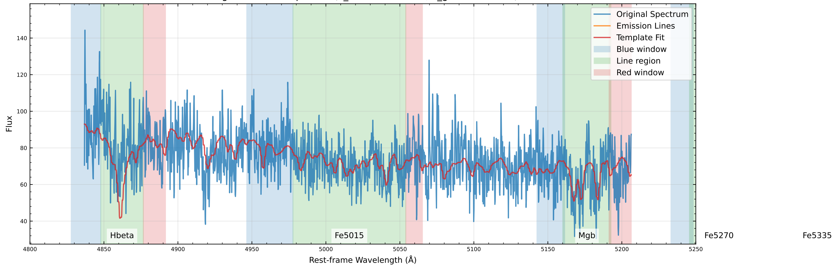
Original Data Comparison (v_star=-16.8 km/s, v_gas=30.8 km/s)
