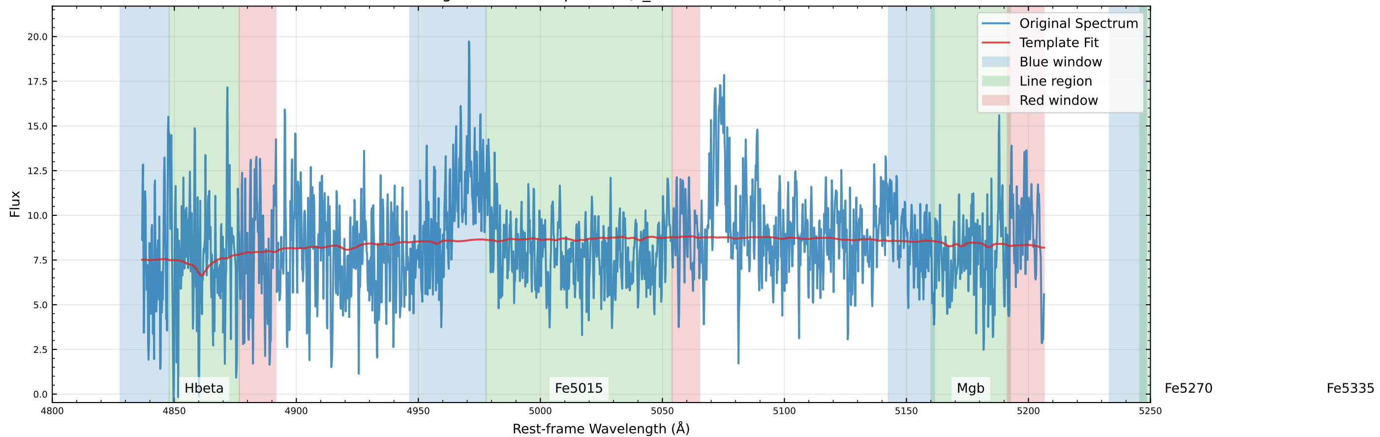
Original Data Comparison (v_star=-35.7 km/s)
