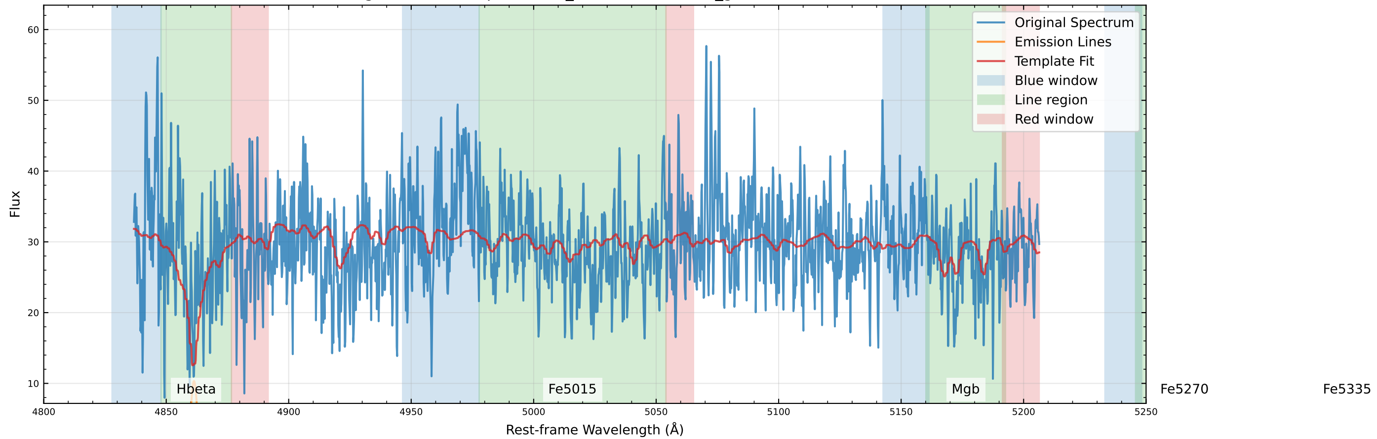
Original Data Comparison (v_star=14.2 km/s, v_gas=92.1 km/s)
