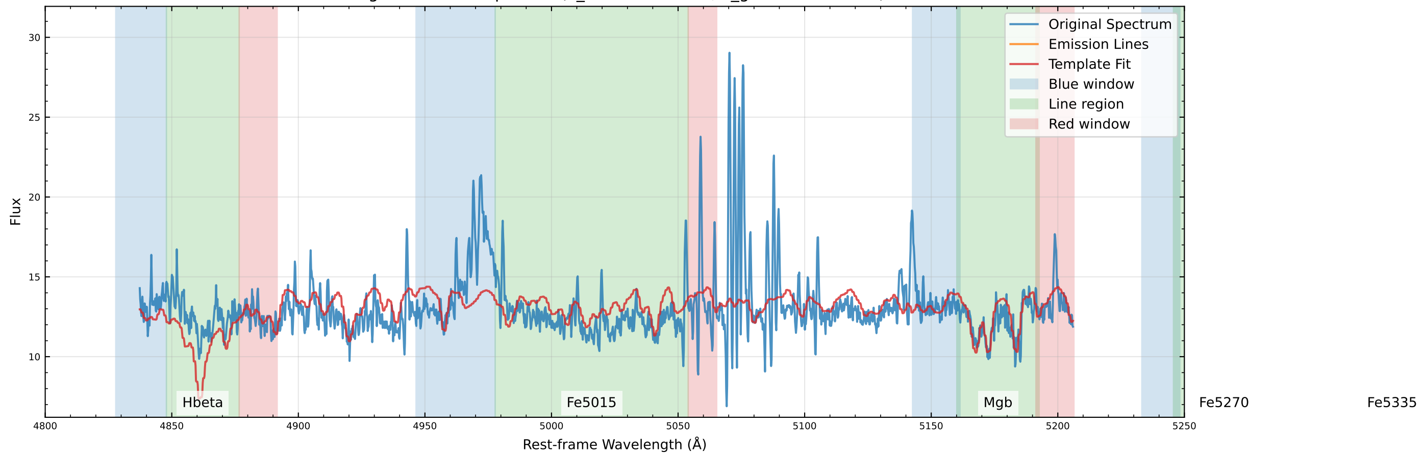
Original Data Comparison (v_star=18.8 km/s, v_gas=-281.2 km/s)
