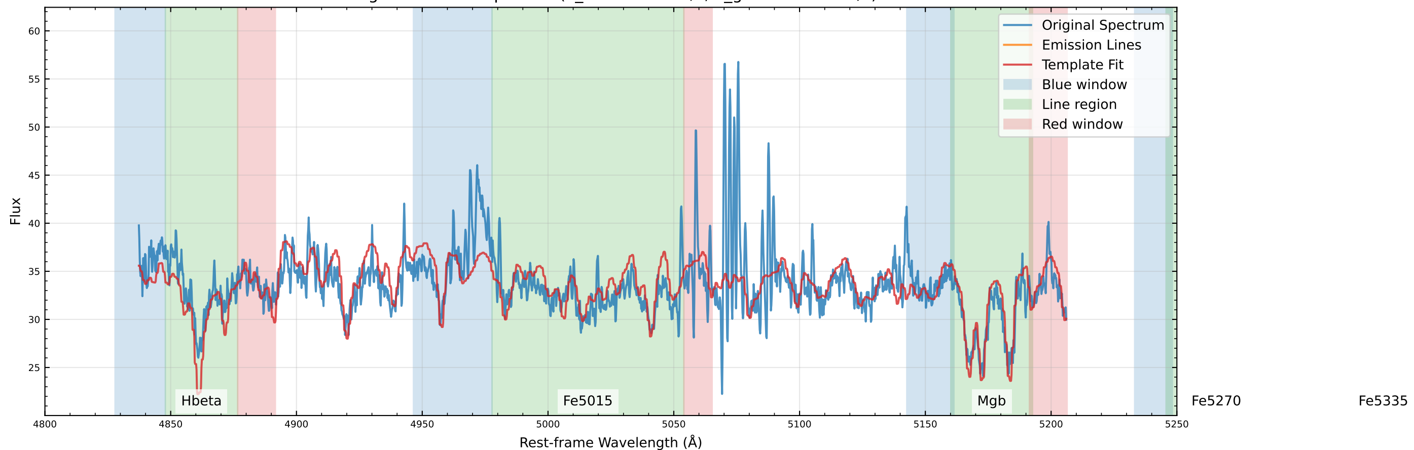
Original Data Comparison (v_star=-1.3 km/s, v_gas=-301.3 km/s)
