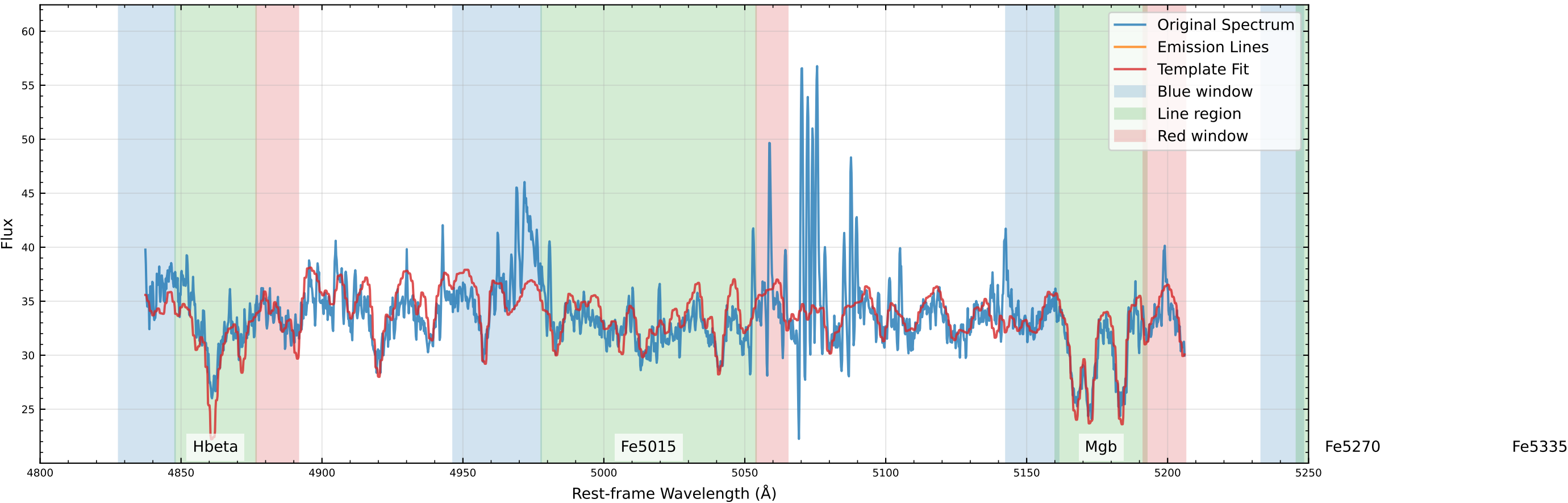
Original Data Comparison (v_star=-1.3 km/s, v_gas=-301.3 km/s)
