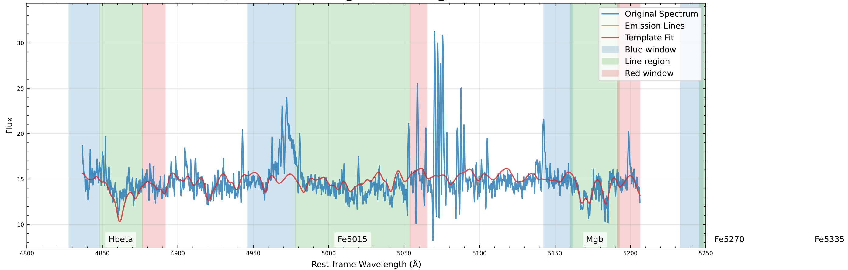
Original Data Comparison (v_star=16.1 km/s, v_gas=-14.2 km/s)
