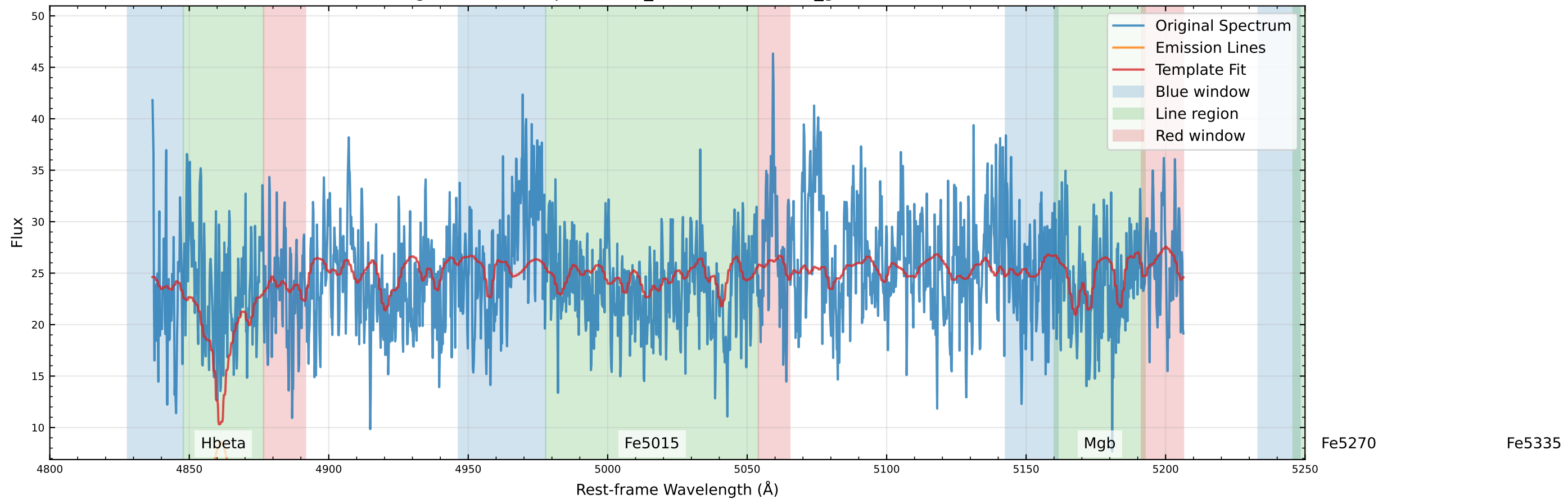
Original Data Comparison (v_star=59.5 km/s, v_gas=44.9 km/s)
