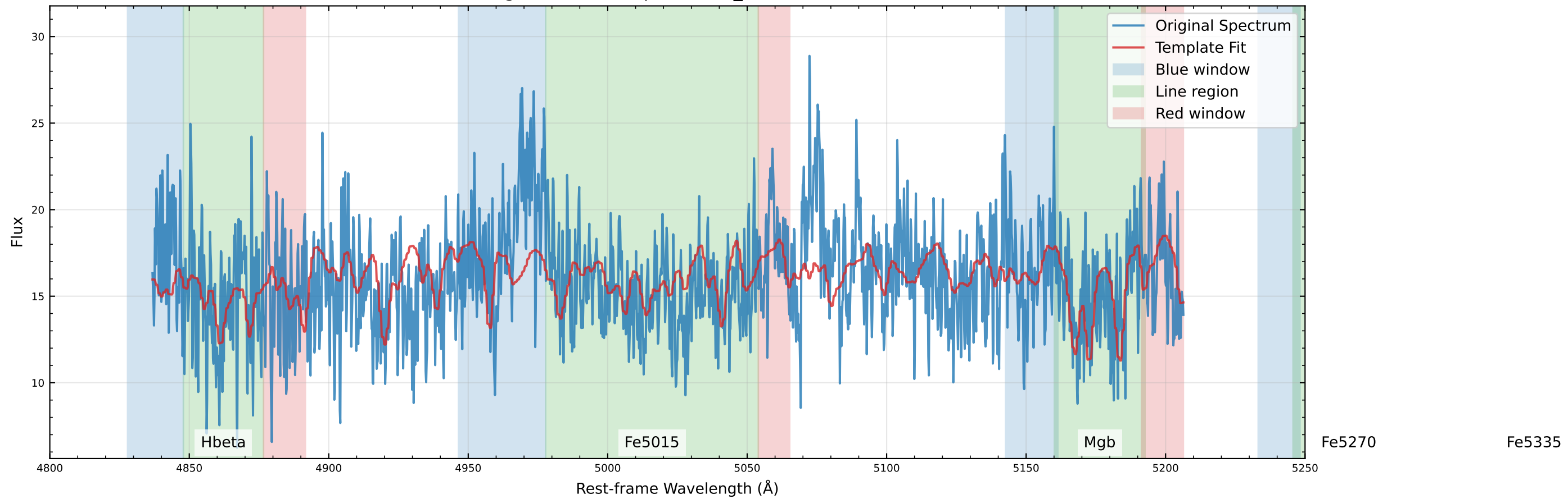
Original Data Comparison (v_star=0.3 km/s)
