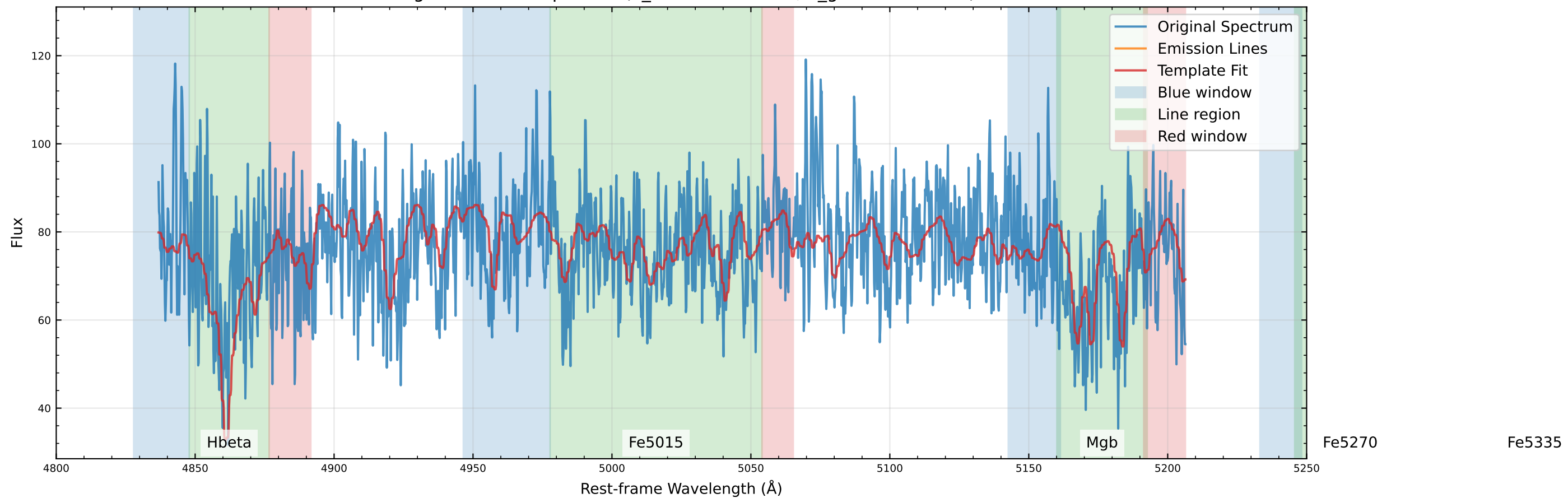
Original Data Comparison (v_star=-36.7 km/s, v_gas=-24.2 km/s)
