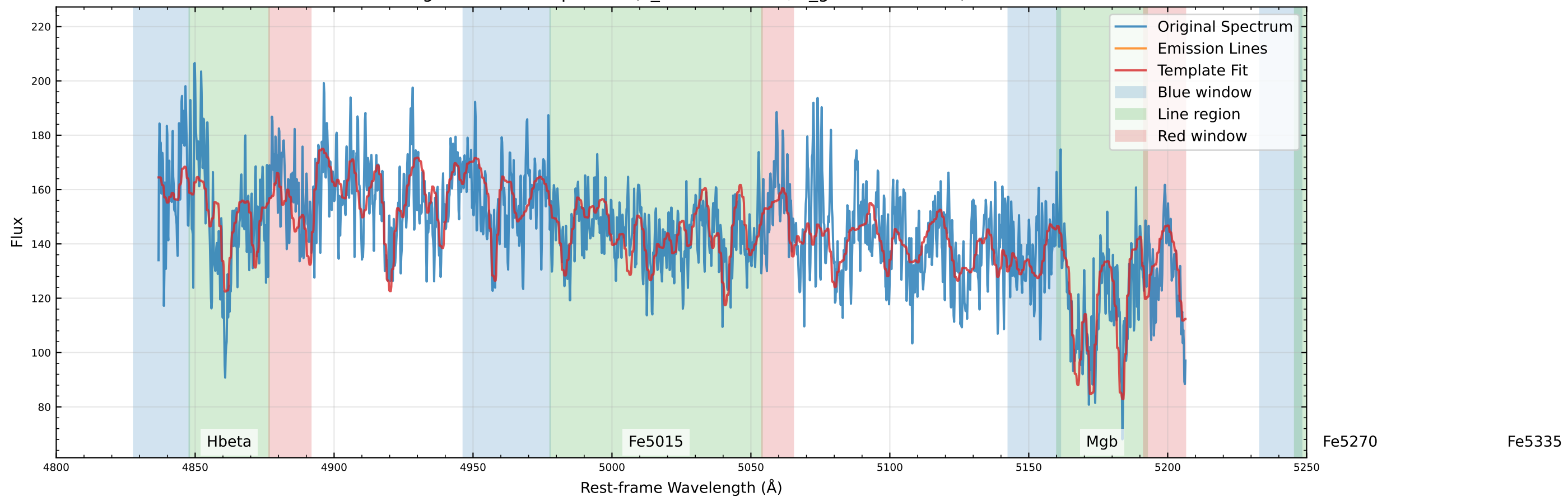
Original Data Comparison (v_star=9.4 km/s, v_gas=-58.1 km/s)
