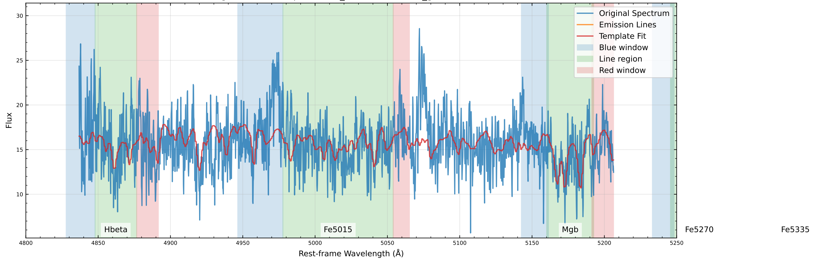
Original Data Comparison (v_star=9.6 km/s, v_gas=4.5 km/s)
