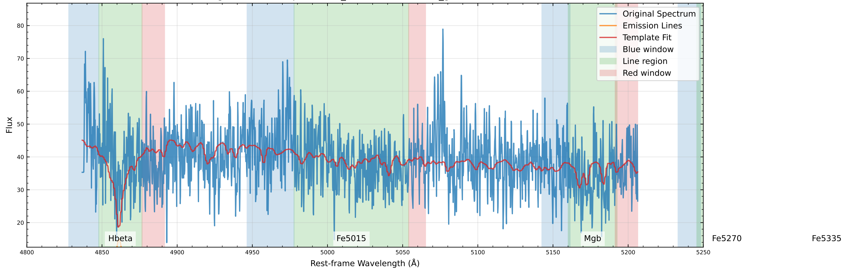
Original Data Comparison (v_star=131.5 km/s, v_gas=251.1 km/s)
