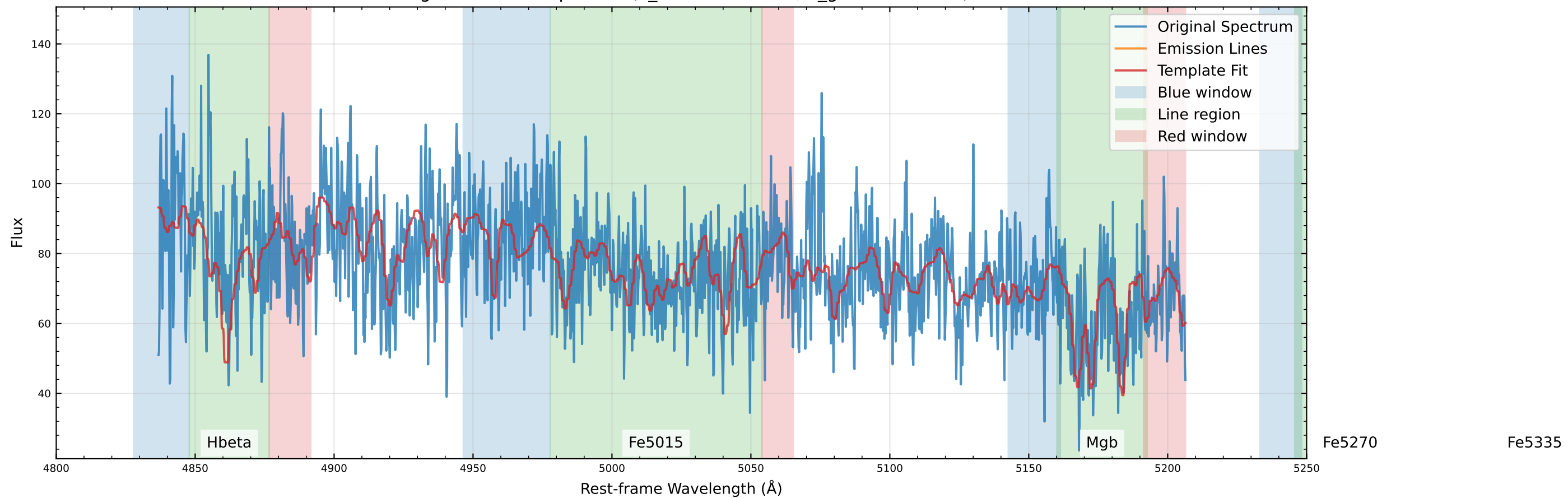
Original Data Comparison (v_star=16.8 km/s, v_gas=35.4 km/s)
