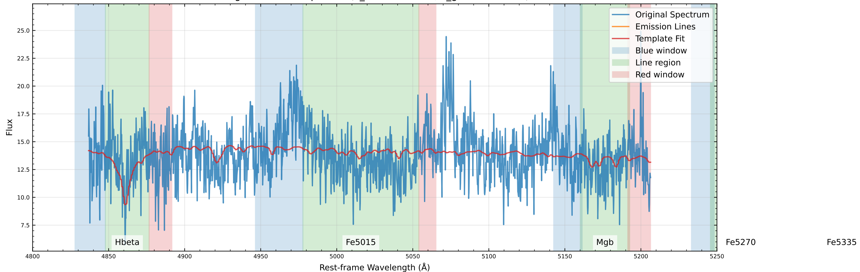
Original Data Comparison ( v_{\text{star}}=9.6 km/s, v_{\text{gas}}=64.6 km/s)
