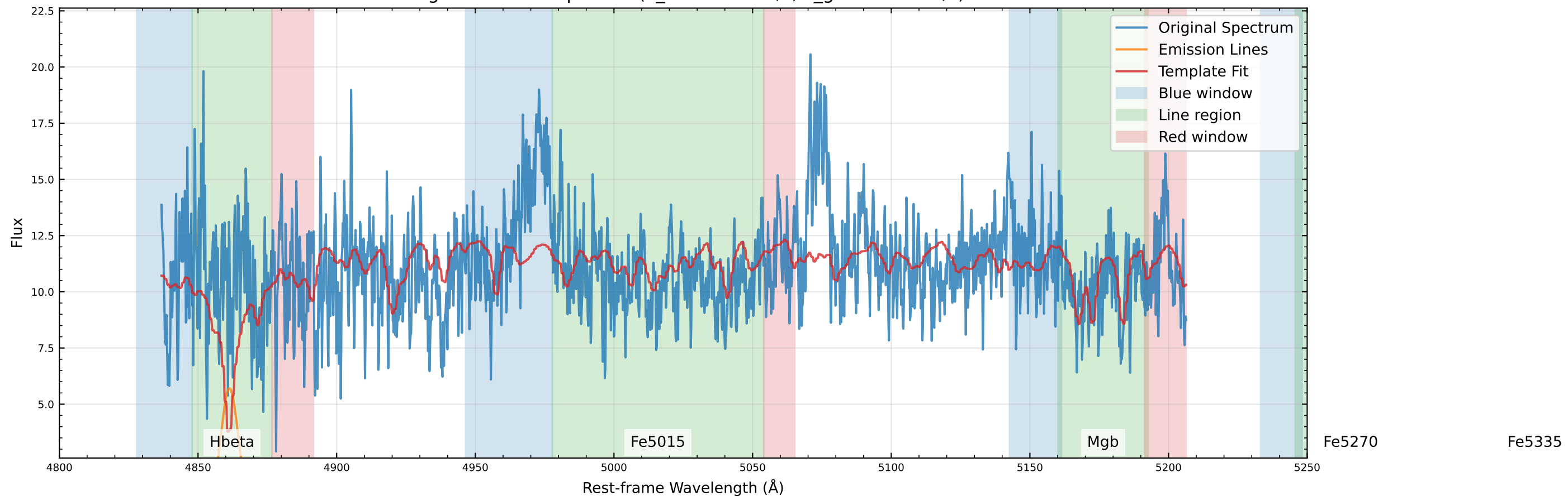
Original Data Comparison (v_star=1.1 km/s, v_gas=32.4 km/s)
