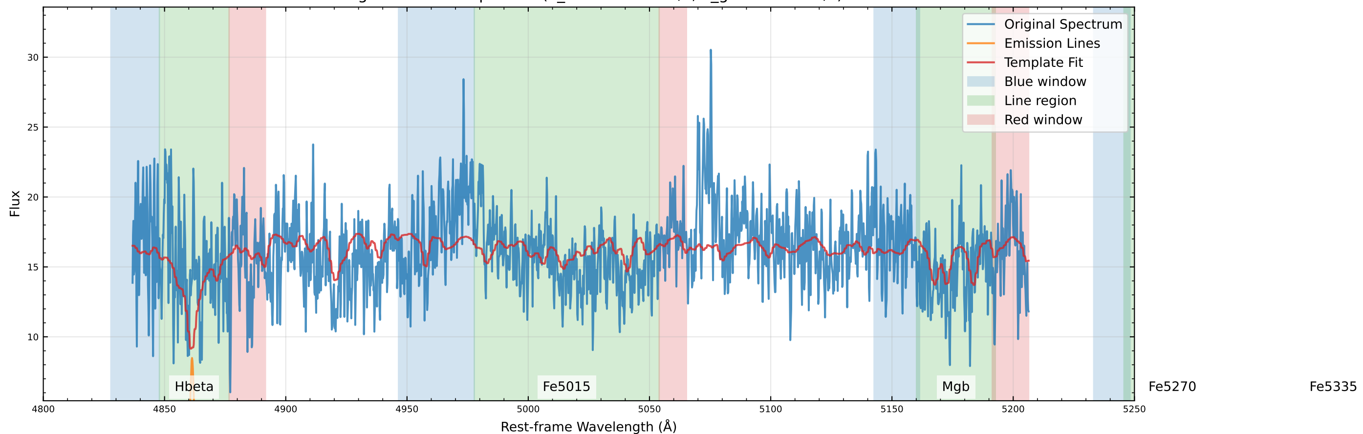
Original Data Comparison (v_star=-25.8 km/s, v_gas=34.3 km/s)
