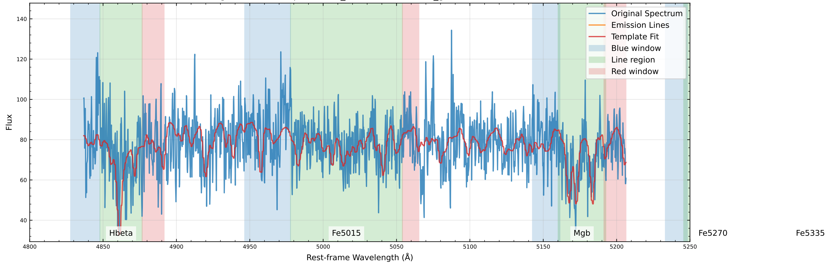
Original Data Comparison (v_star=-20.1 km/s, v_gas=22.8 km/s)
