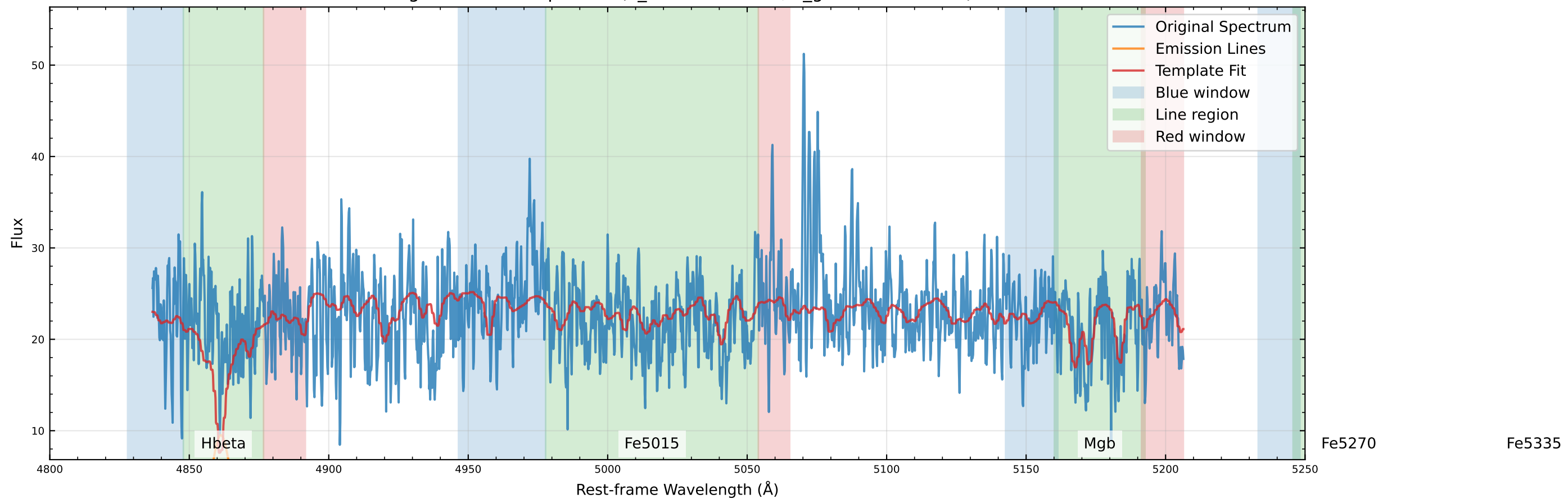
Original Data Comparison (v_star=-3.6 km/s, v_gas=-122.7 km/s)
