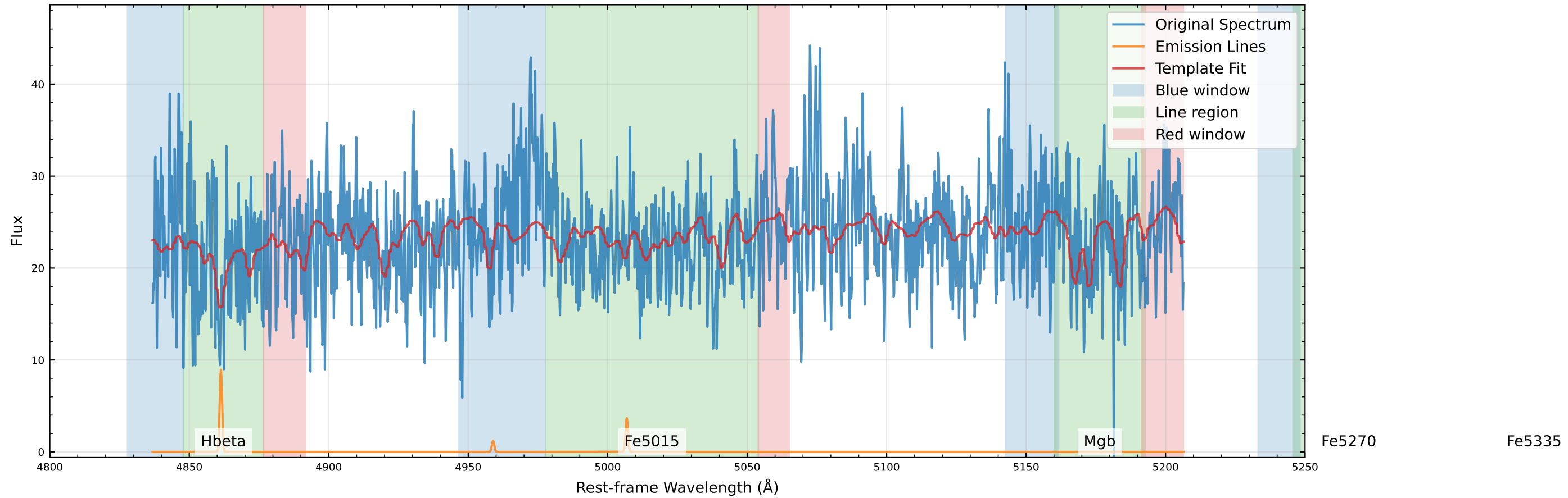
Original Data Comparison ( v_{\text{star}}=35.0 km/s, v_{\text{gas}}=120.3 km/s)
