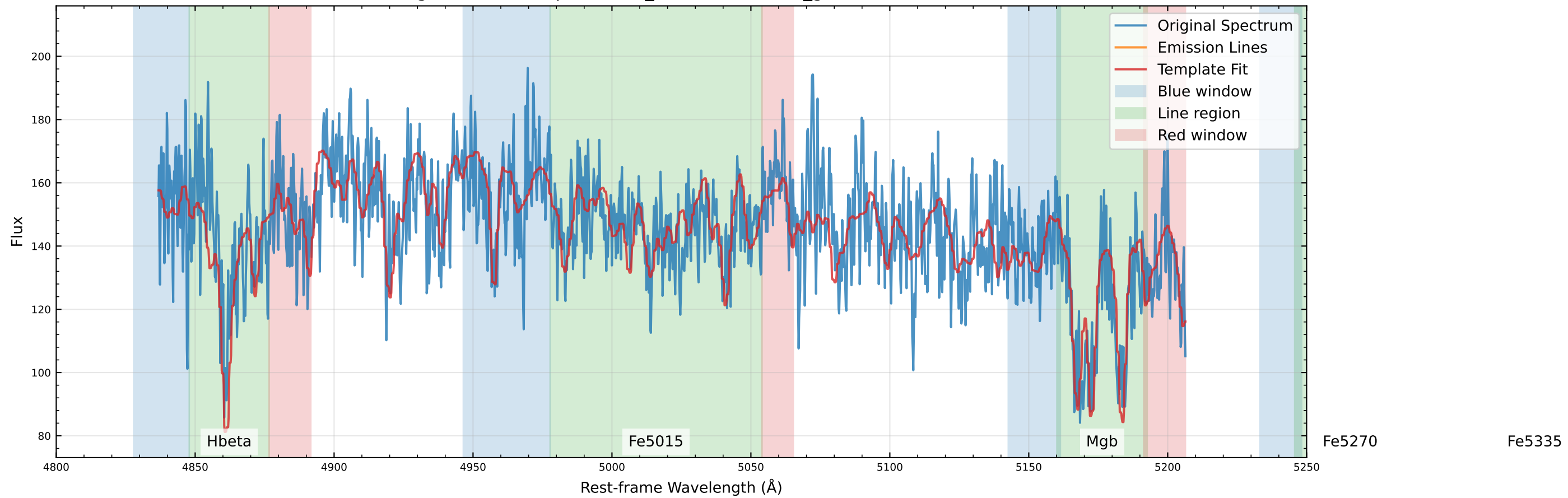
Original Data Comparison (v_star=7.3 km/s, v_gas=-292.7 km/s)
