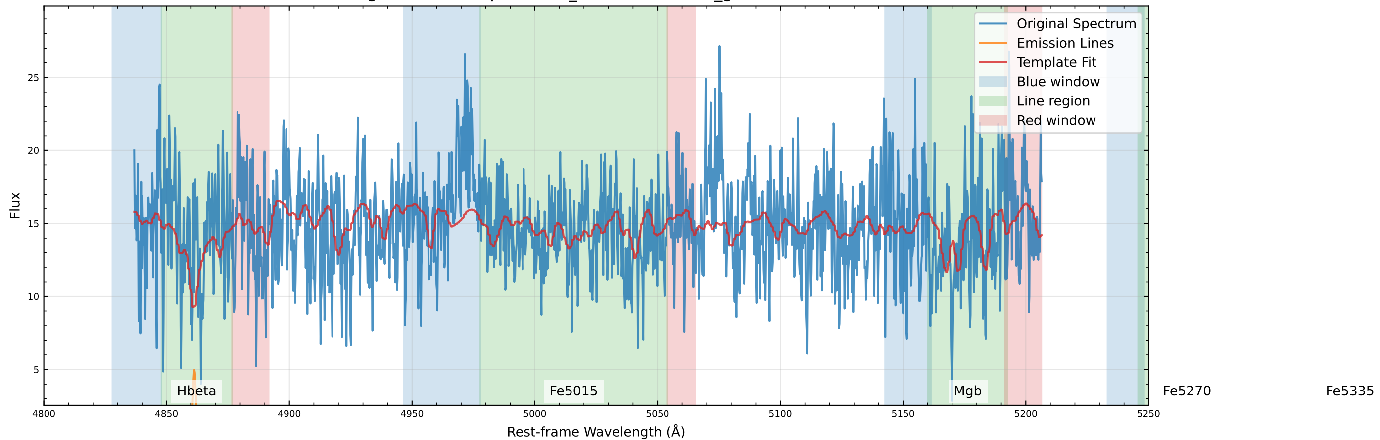
Original Data Comparison (v_star=-8.4 km/s, v_gas=25.8 km/s)
