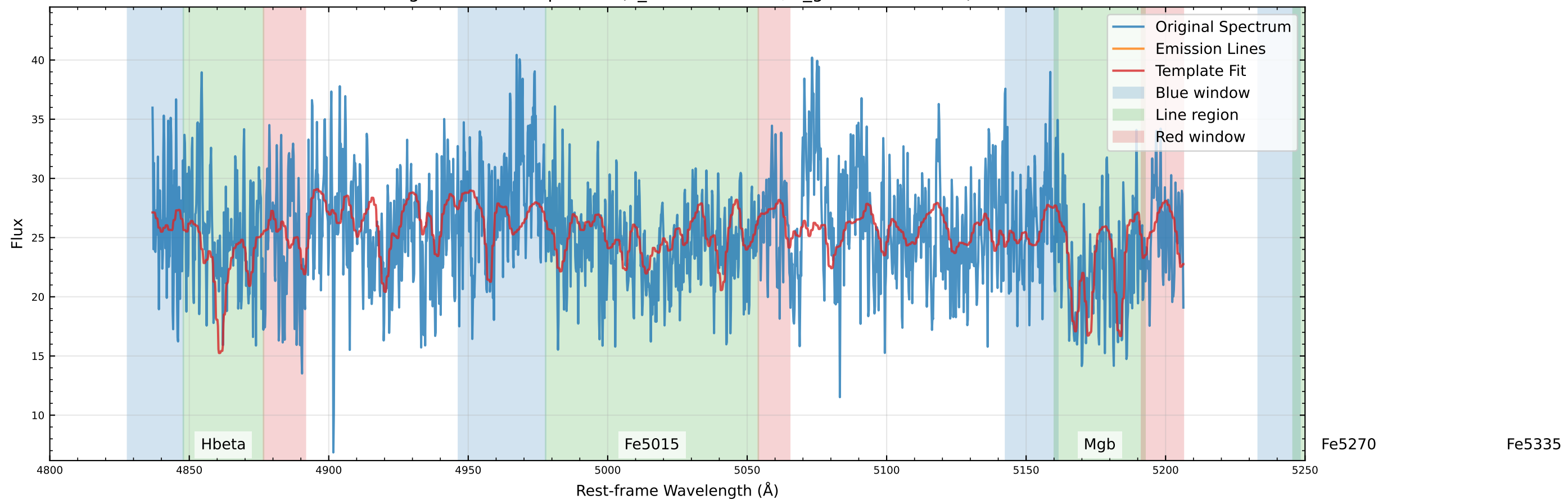
Original Data Comparison (v_star=-7.2 km/s, v_gas=-184.5 km/s)
