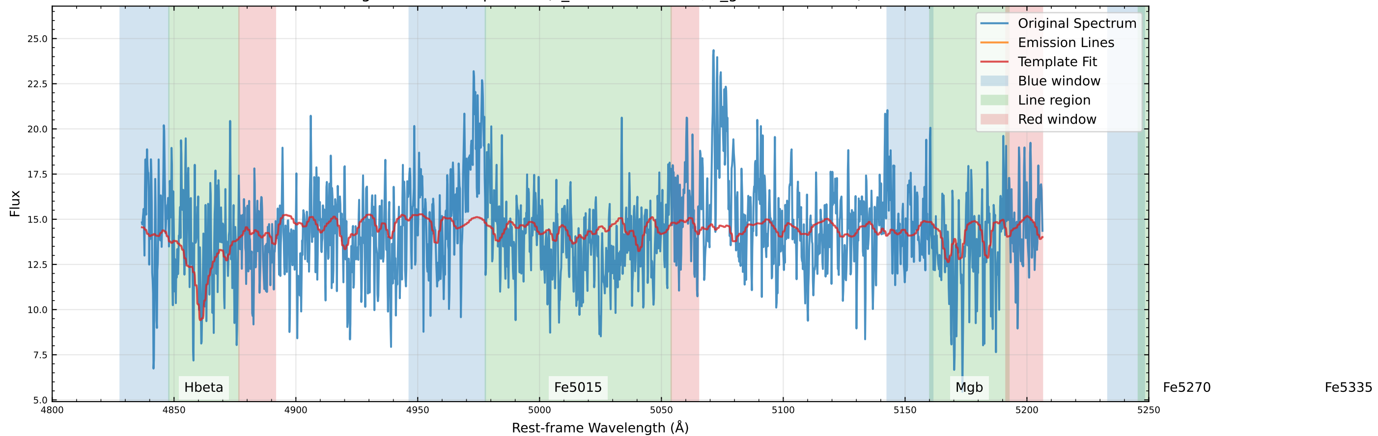
Original Data Comparison (v_star=137.5 km/s, v_gas=156.5 km/s)
