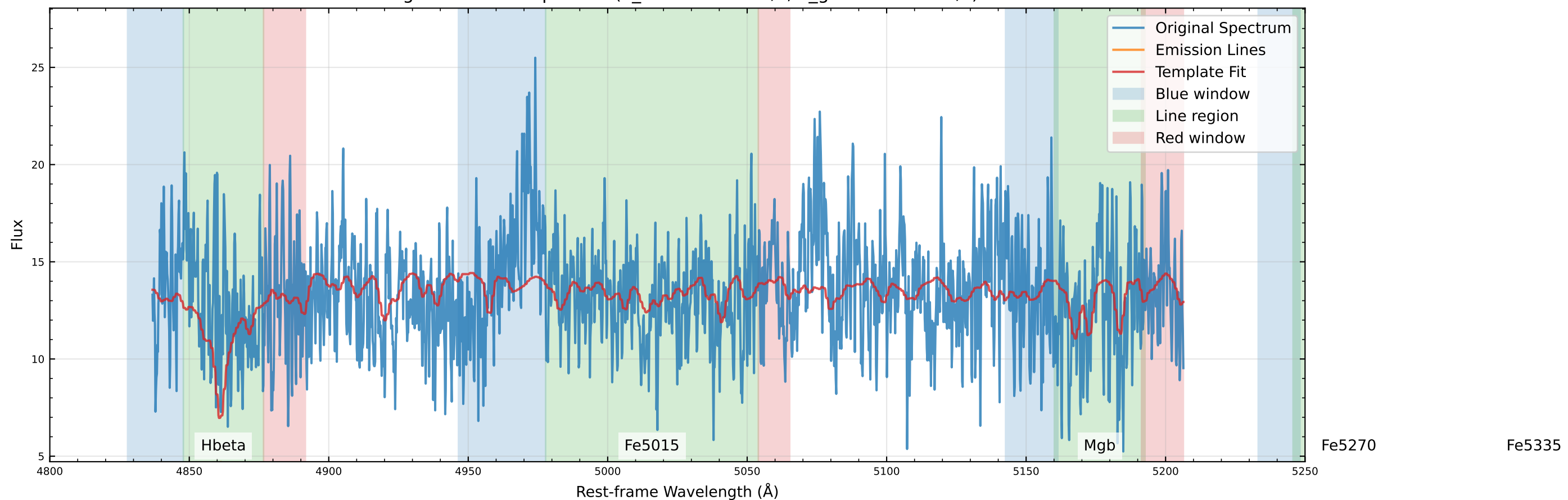
Original Data Comparison (v_star=-17.7 km/s, v_gas=-101.0 km/s)
