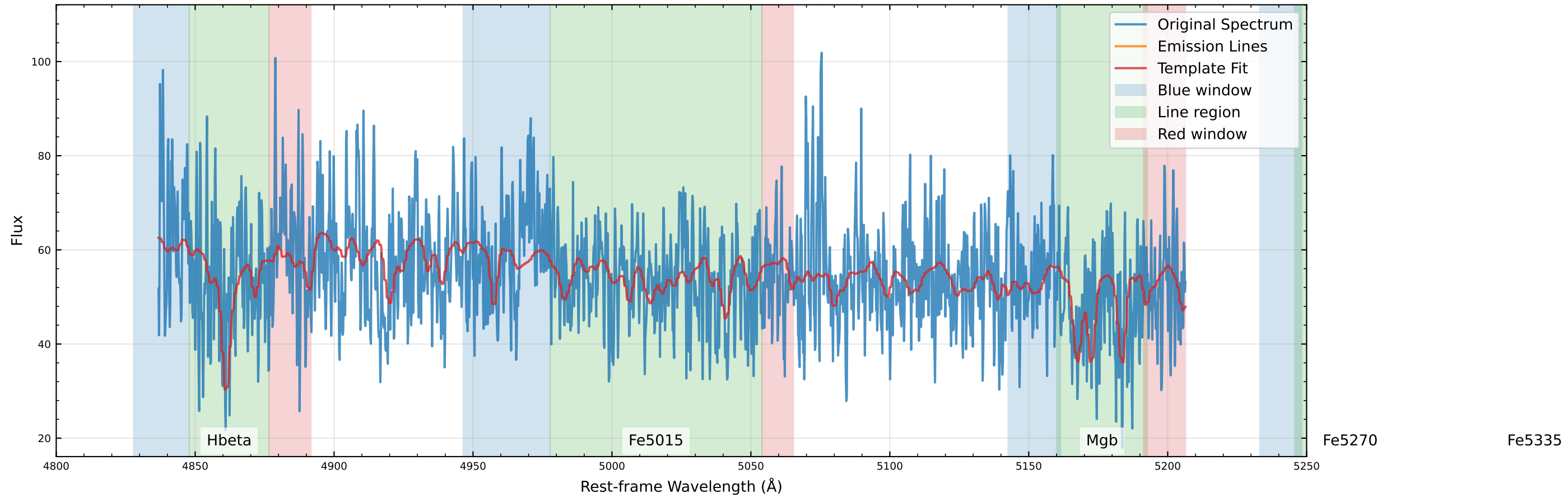
Original Data Comparison (v_star=-2.1 km/s, v_gas=11.8 km/s)
