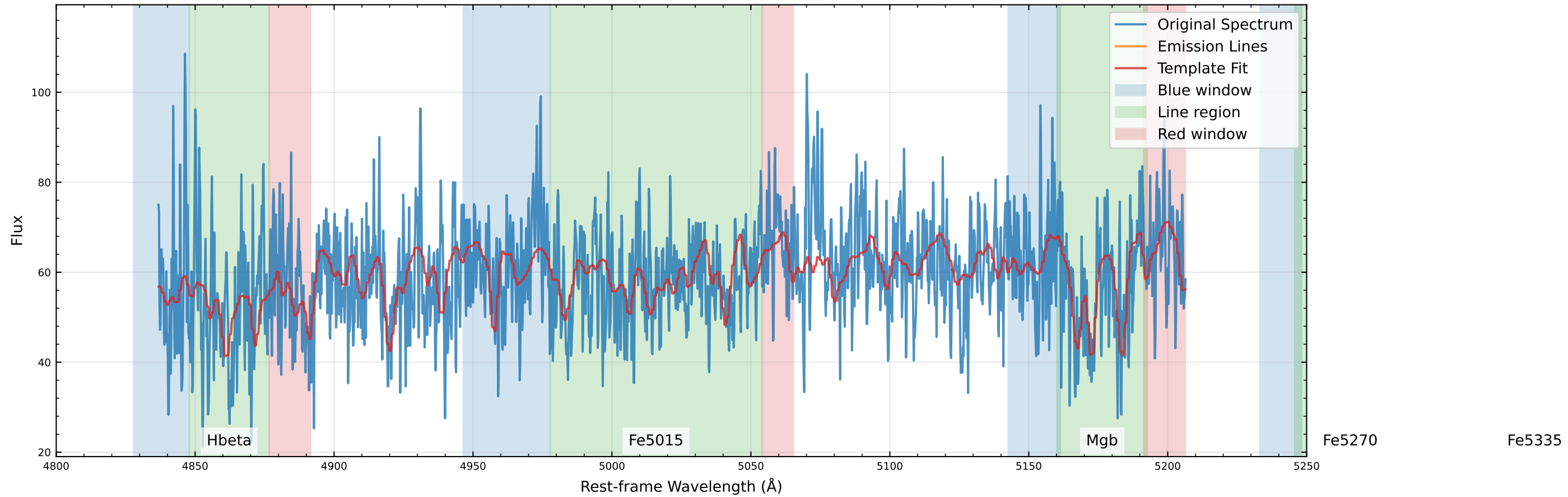
Original Data Comparison (v_star=3.4 km/s, v_gas=-12.9 km/s)
