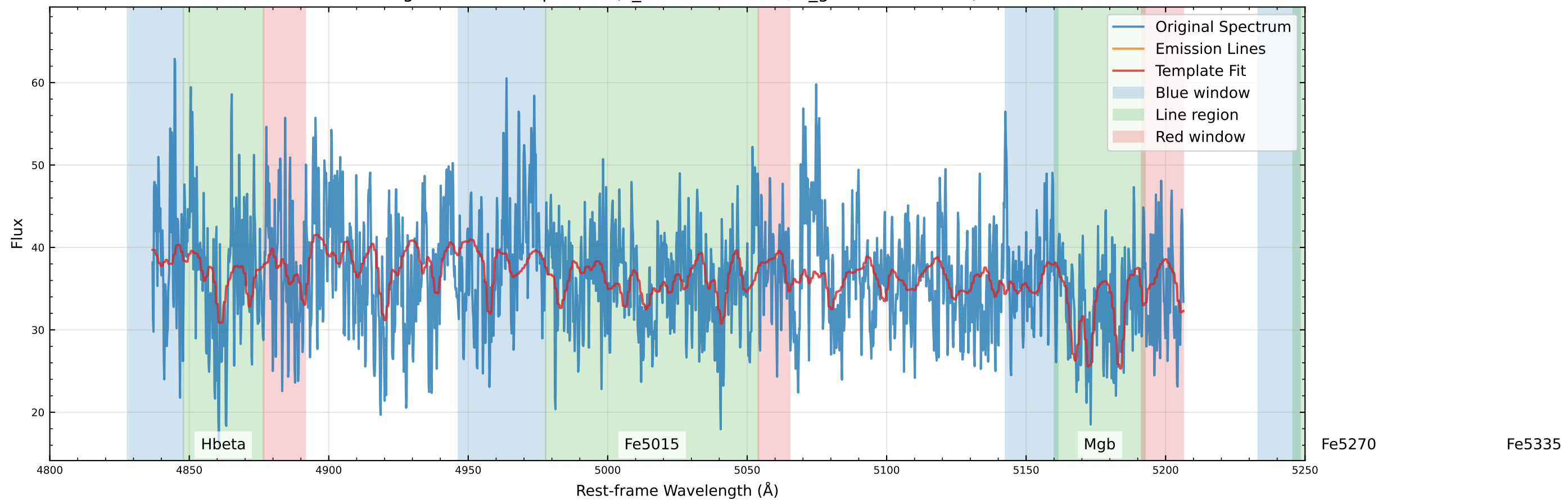
Original Data Comparison (v_star=-39.0 km/s, v_gas=-175.4 km/s)
