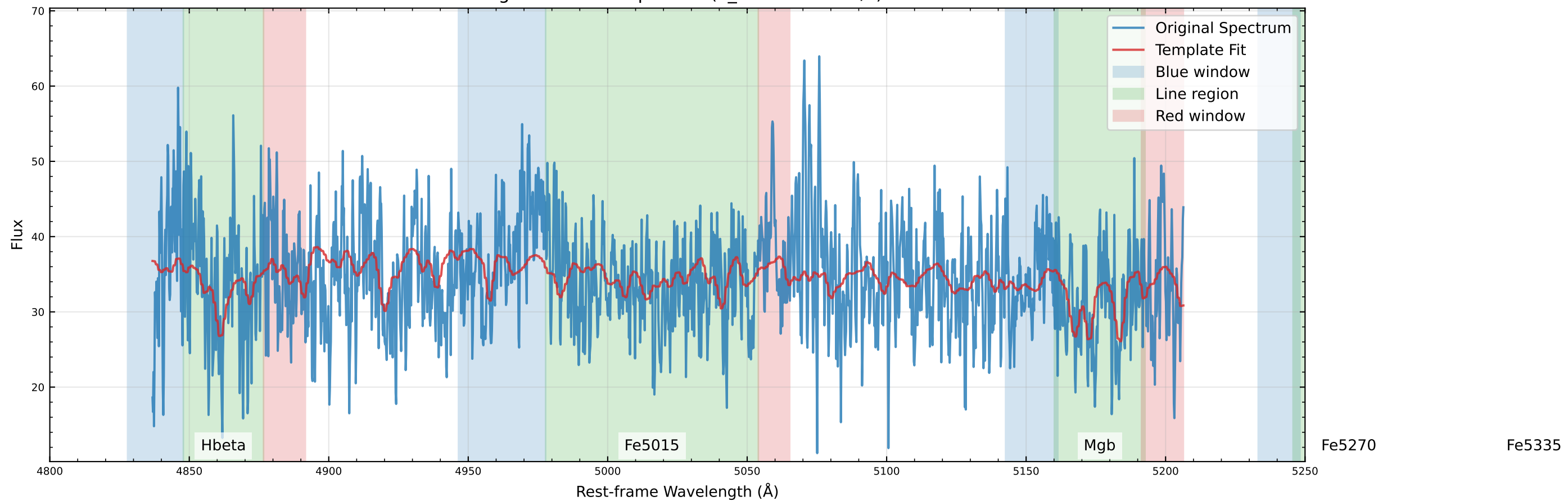
Original Data Comparison (v_star=40.6 km/s)
