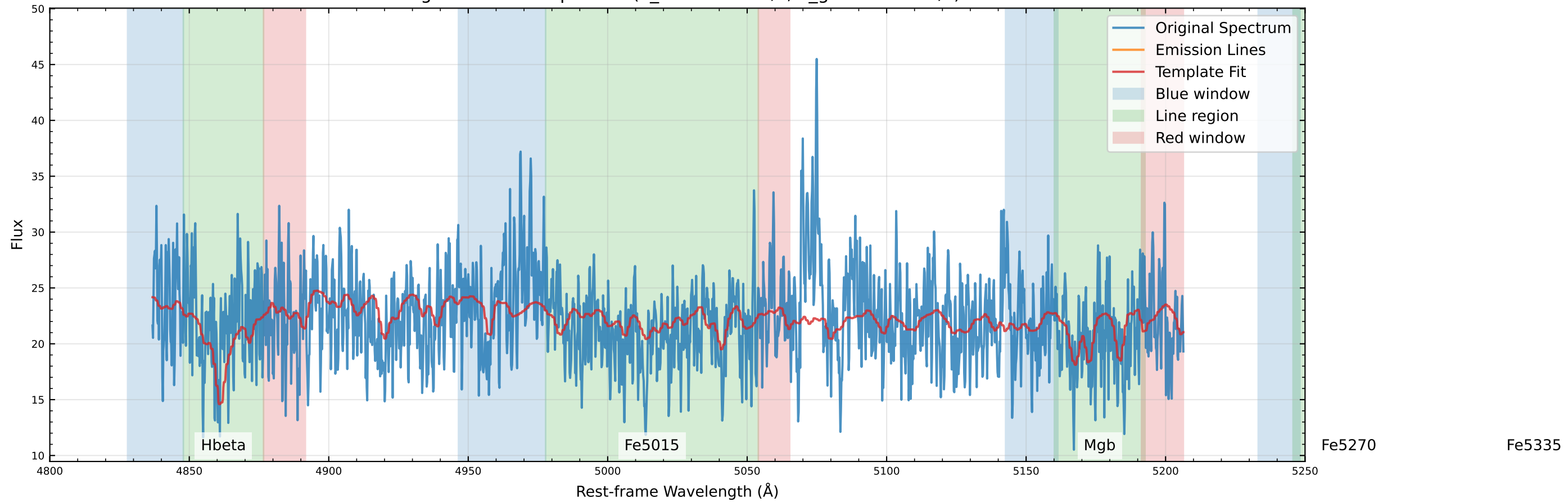
Original Data Comparison (v_star=9.2 km/s, v_gas=52.2 km/s)
