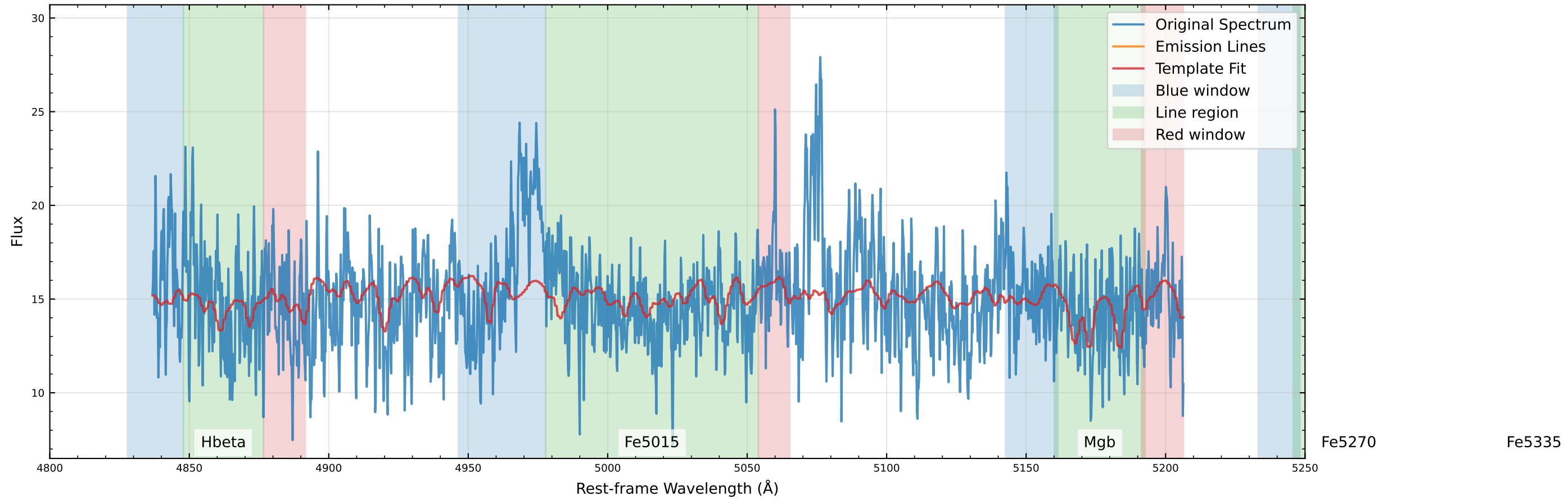
Original Data Comparison (v_star=75.4 km/s, v_gas=76.2 km/s)
