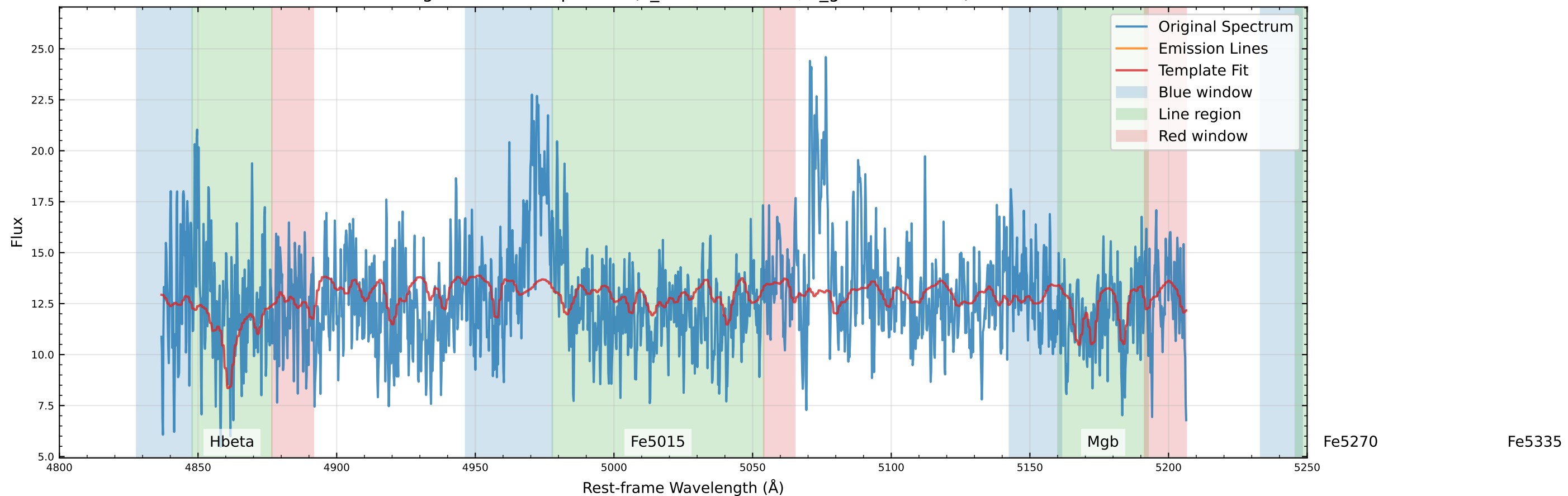
Original Data Comparison (v_star=51.3 km/s, v_gas=51.7 km/s)
