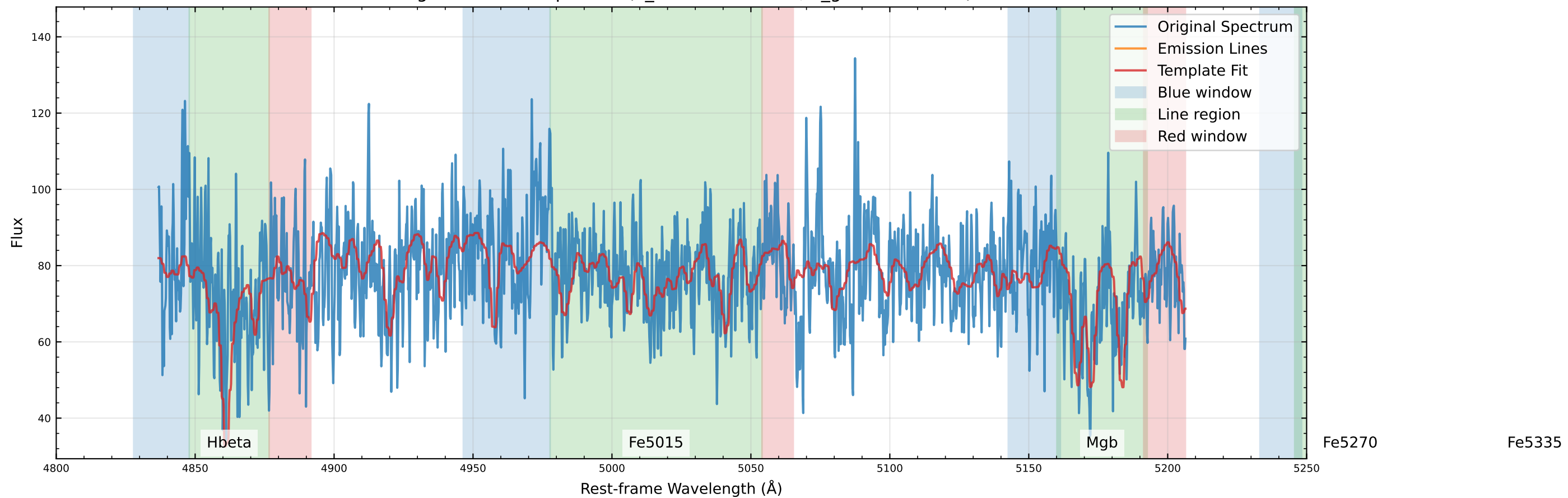
Original Data Comparison ( v_{\text{star}}=-20.1 km/s, v_{\text{gas}}=22.8 km/s)
