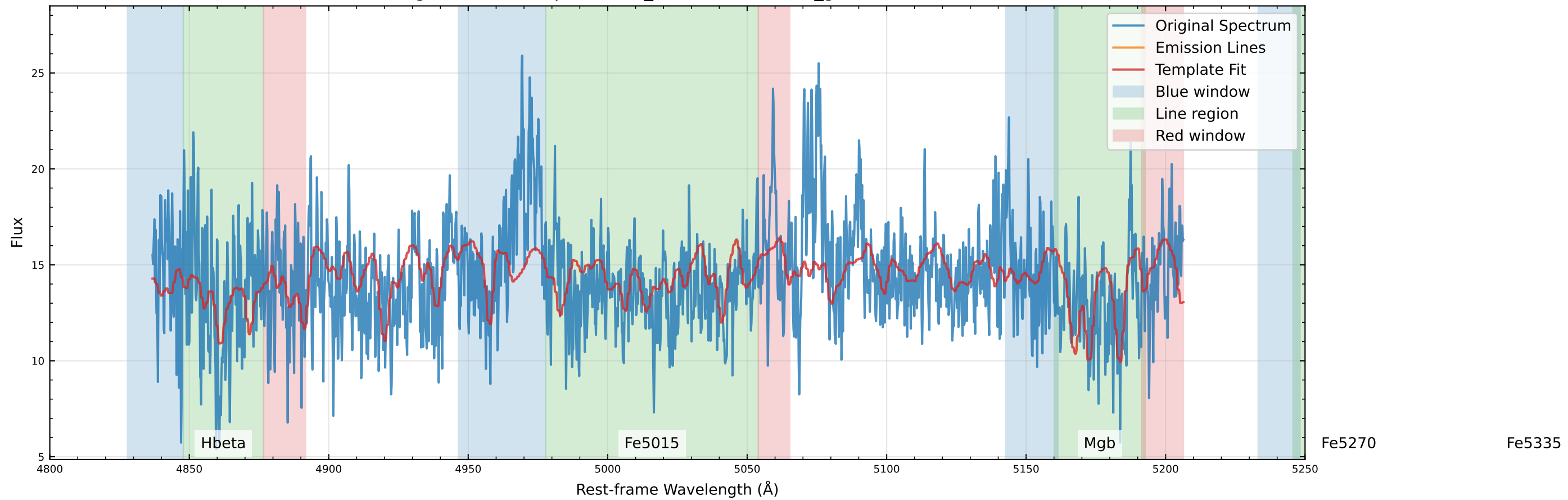
Original Data Comparison (v_star=32.3 km/s, v_gas=73.0 km/s)
