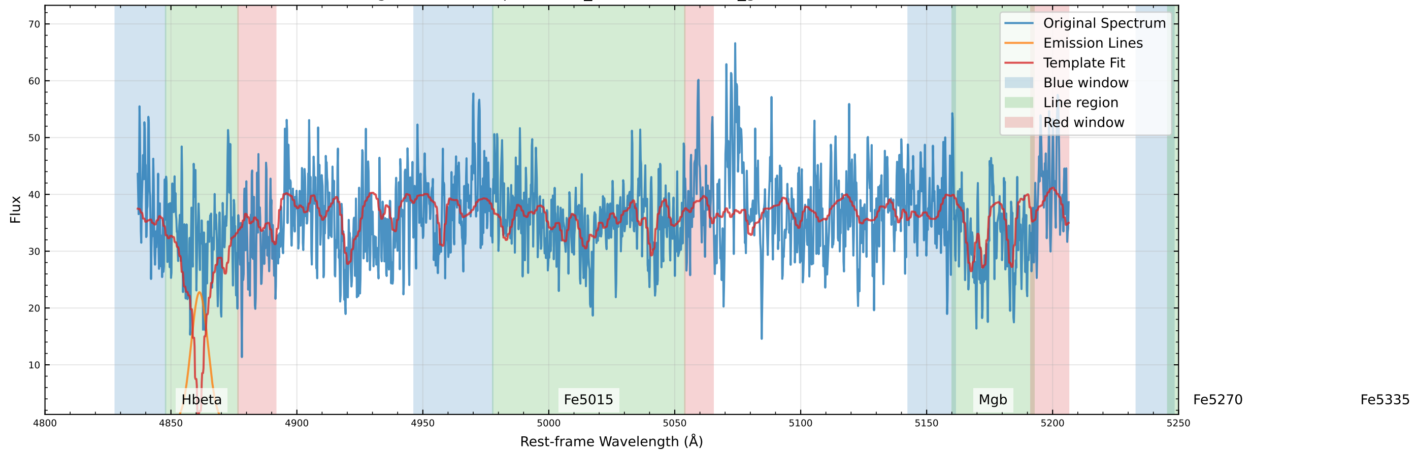
Original Data Comparison (v_star=37.1 km/s, v_gas=-3.7 km/s)
