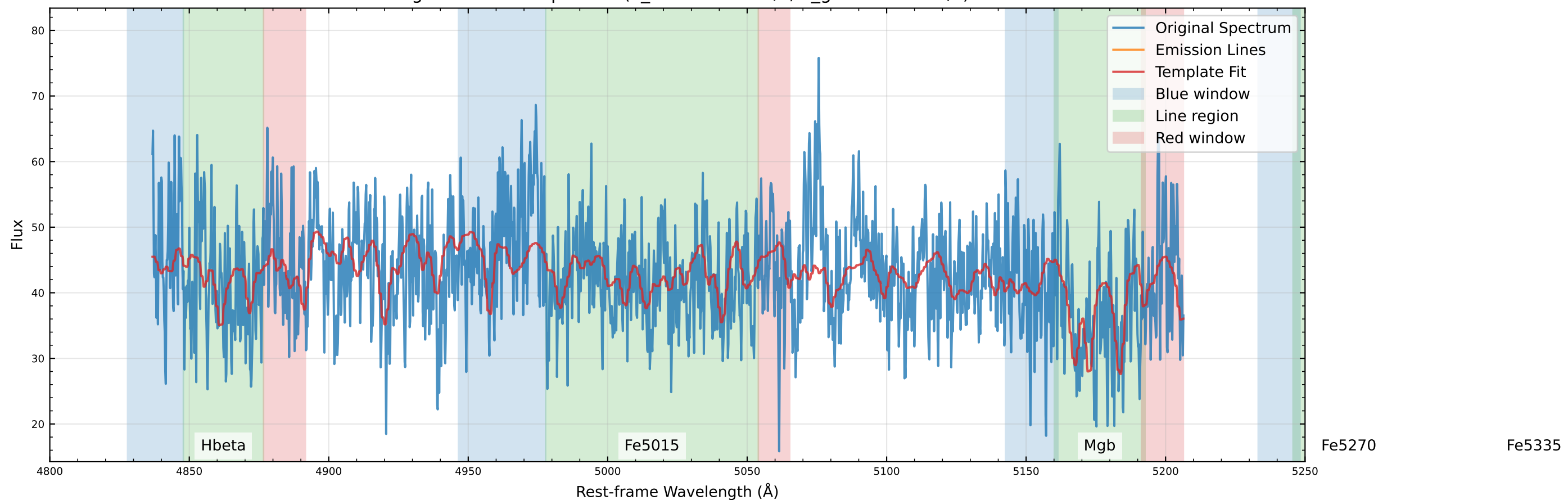
Original Data Comparison (v_star=31.4 km/s, v_gas=-42.4 km/s)
