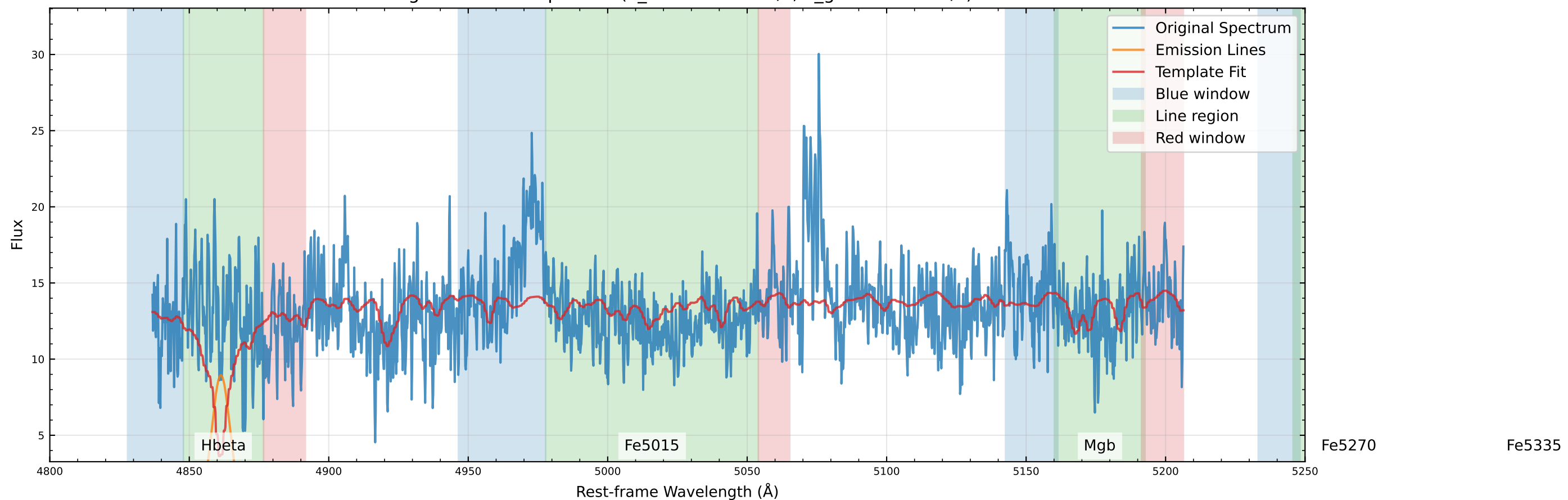
Original Data Comparison (v_star=-11.8 km/s, v_gas=-48.4 km/s)
