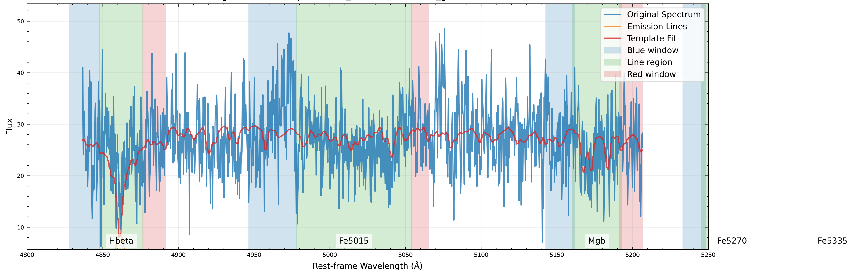
Original Data Comparison (v_star=-6.1 km/s, v_gas=-143.2 km/s)
