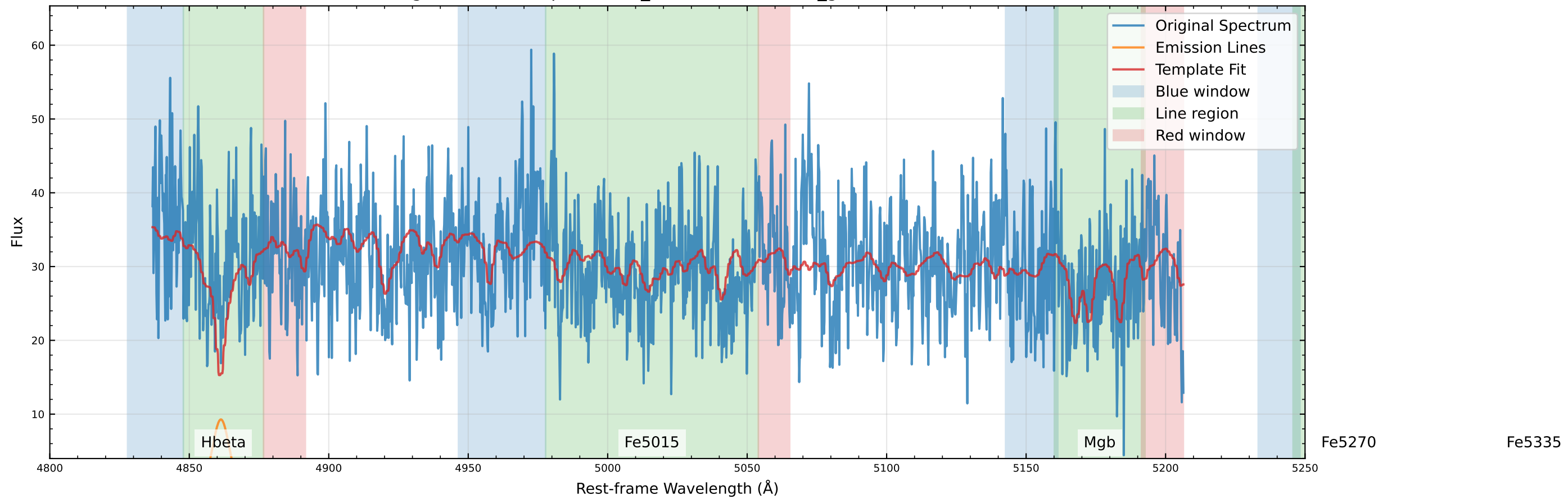
Original Data Comparison (v_star=-16.2 km/s, v_gas=55.3 km/s)
