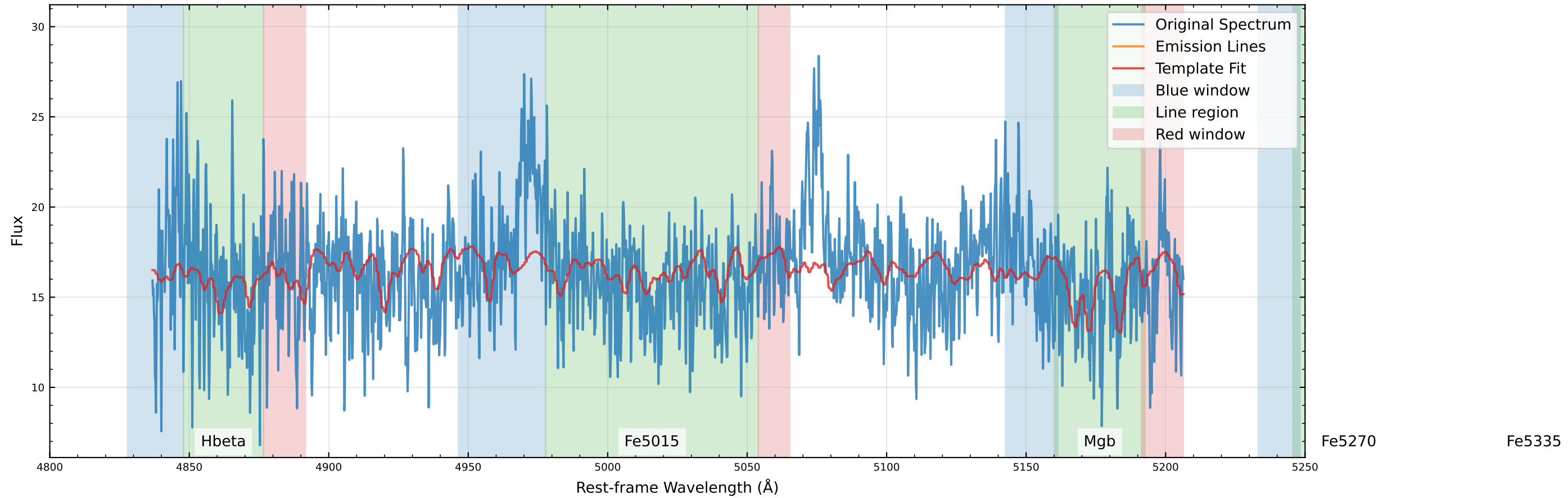
Original Data Comparison (v_star=18.8 km/s, v_gas=-55.1 km/s)
