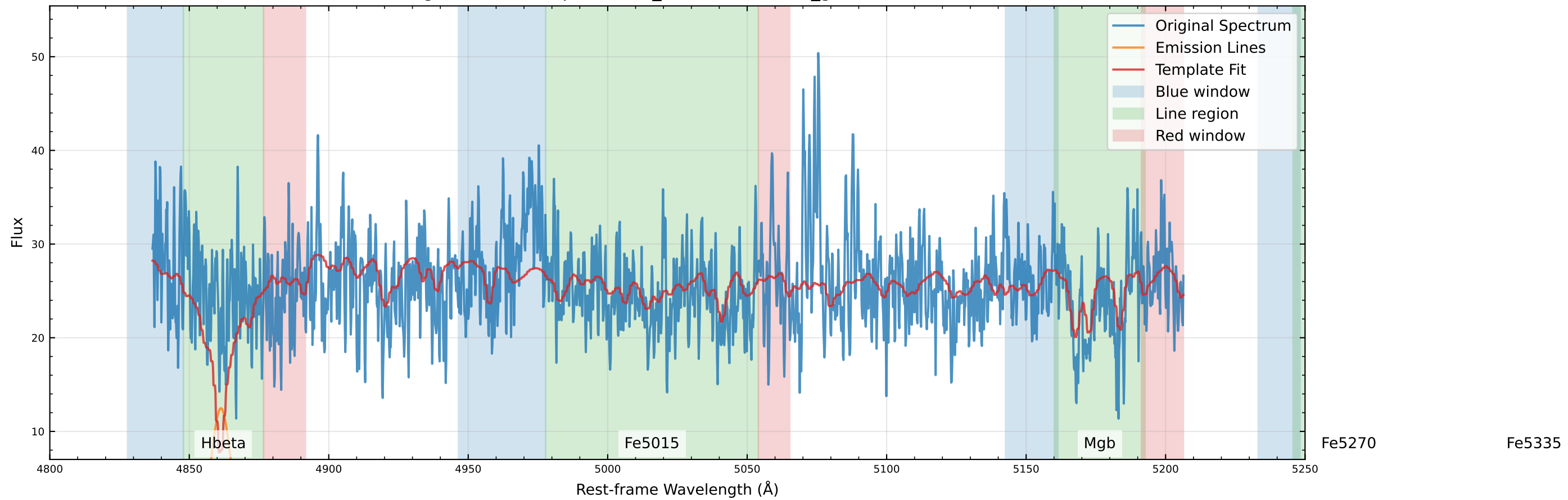
Original Data Comparison (v_star=8.8 km/s, v_gas=-0.9 km/s)
